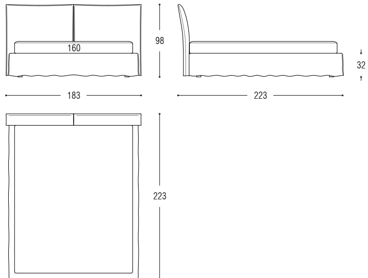
Bed for slat cm 160x200
