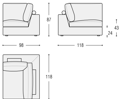
Corner element cm 120x100 right
